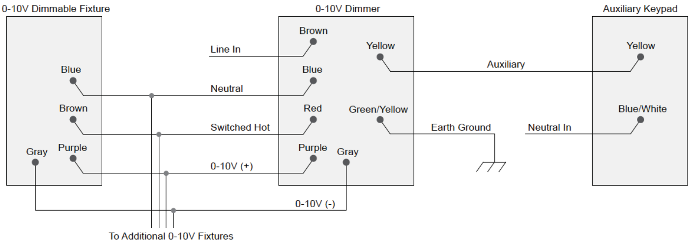
Figure 3. Multiple Device Location Using Auxiliary Keypad, With Neutral Connection
