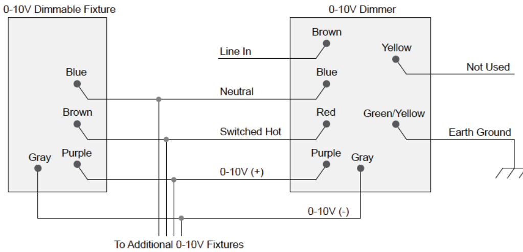
Figure 2. Single Device Location, With Neutral Connection
