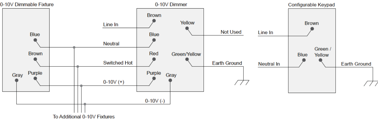
Figure 4. Multiple Device Location Using Configurable Keypad, Neutral Required
